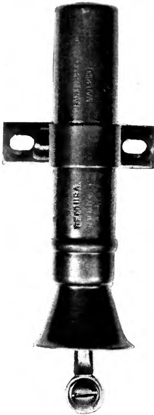
Fig. 2. One of the latest types of vacuum-gap lightning arresters is illustrated here. Its internal construction is shown in the accompanying sketch
